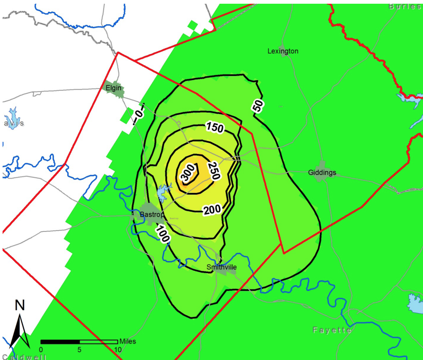
Project specific 50year drawdown (in feet) in the Simsboro Aquifer attributable to the proposed LCRA pumpage estimated using the GAM
