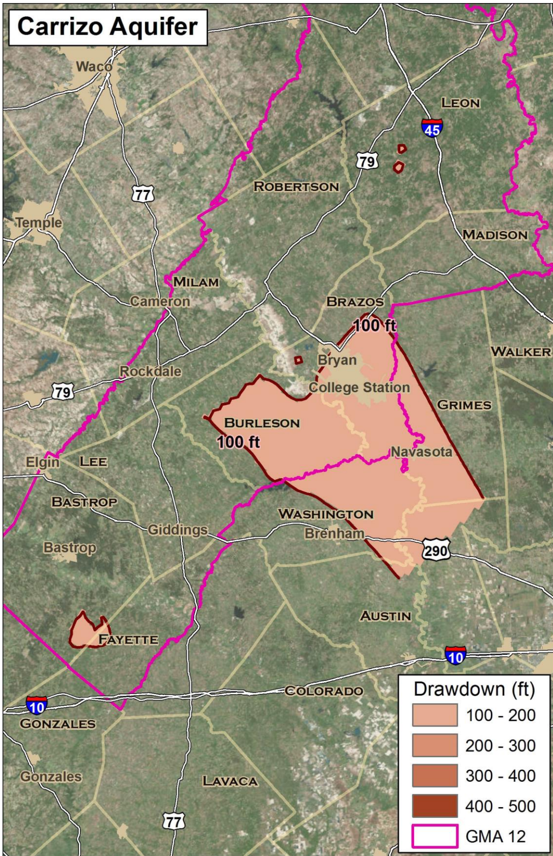
Figure 6 GAM predicted drawdowns in the Carrizo Aquifer due to baseline pumping, 2000 - 2060
