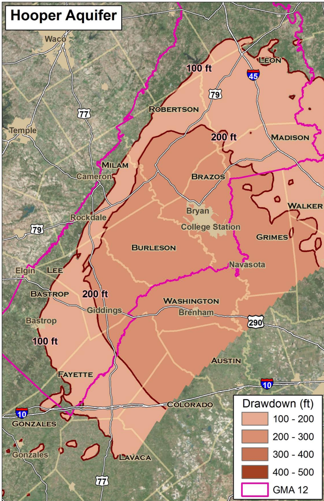
Figure 3 GAM predicted drawdowns in the Hooper Aquifer due to baseline pumping, 2000 - 2060
