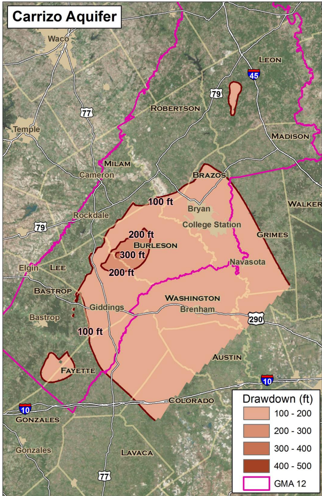
Figure 11 GAM predicted drawdowns in the Carrizo Aquifer due to baseline pumping plus additional pumping by Vista Ridge, End Op, Forstar, and LCRA, 2000 - 2060
